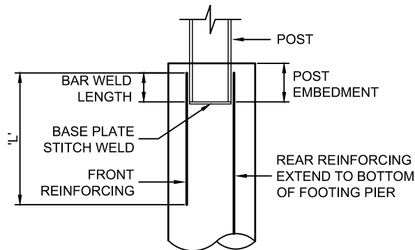
TYPICAL POST BASE DETAIL (H = 0-2550mm)
